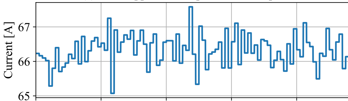
(a) RMS ripple current per DC-link capacitor
