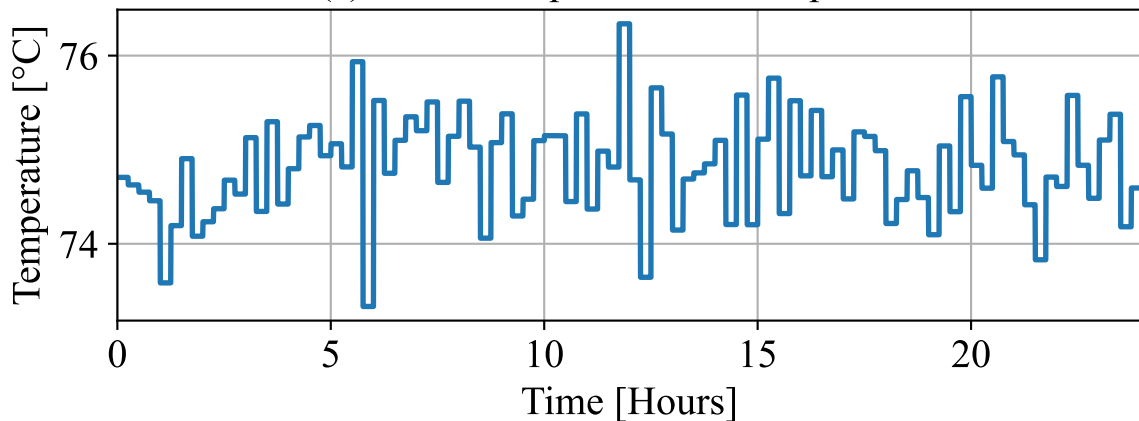
(c) DC-link capacitor core temperature
