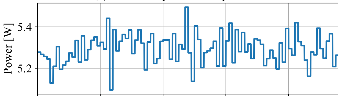
(b) DC-link capacitor total power losses
